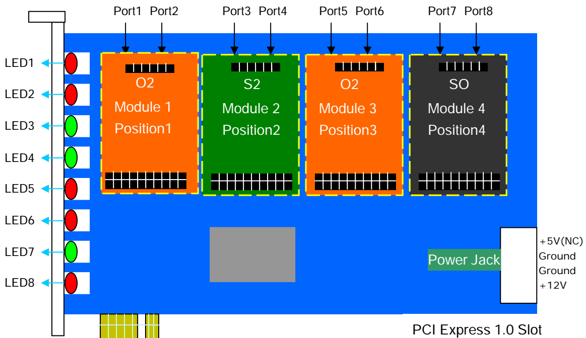
Figure 1: TDM800E Modules
